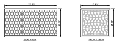
Fig. 8 Make sure the tanks are oriented properly in the excavation.
