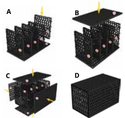
Figure 2 Follow these steps to assemble a 5-plate R-Tank HD ®.
