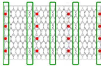
Fig. 1 For standard R-Tank LD ® (4-plate) projects, attach small plates at locations with red dots. For R-Tank HD ® and R-Tank SD ® (5-plate) projects, attach small plates at locations circled in green.
