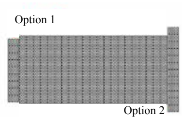
Fig. 10 Plan view showing the end rows turned perpendicular. The corners may not match up perfectly, so two acceptable alternatives are shown. Most plans do not show this configuration. Field adjustments are easily made.
