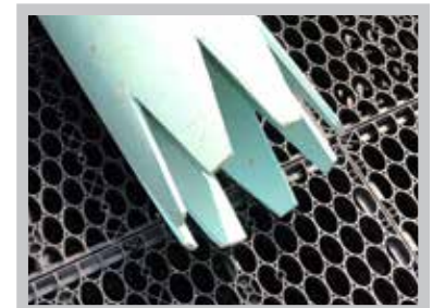
Fig. 14 Cut 8" notches into the bottom of Maintenance Port.
