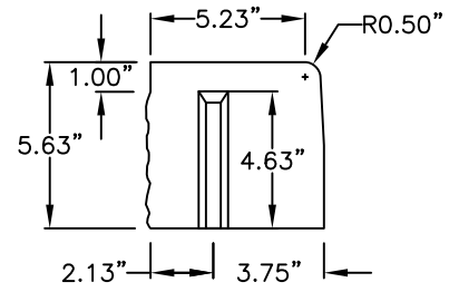
SIDE VIEW "A"
